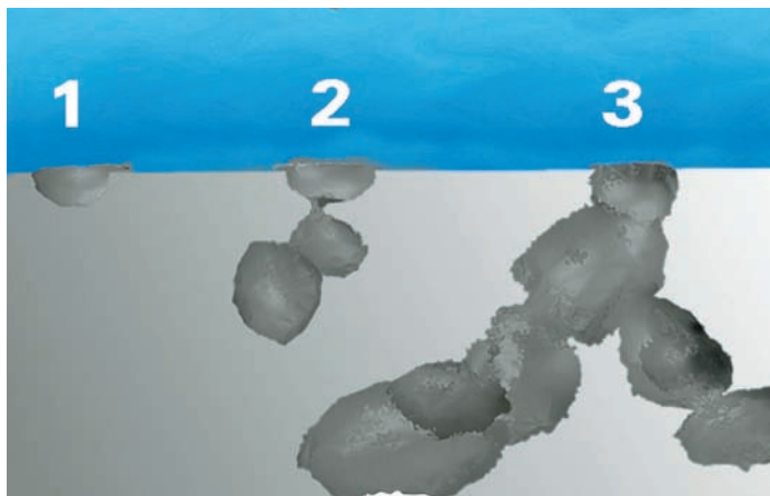
The stages of corrosion: 1. Initial Pit forms; 2. Auto catalytic process speeds up as concentrated solution becomes more aggressive; 3. Leak occurs as pit breaks through outer surface.
